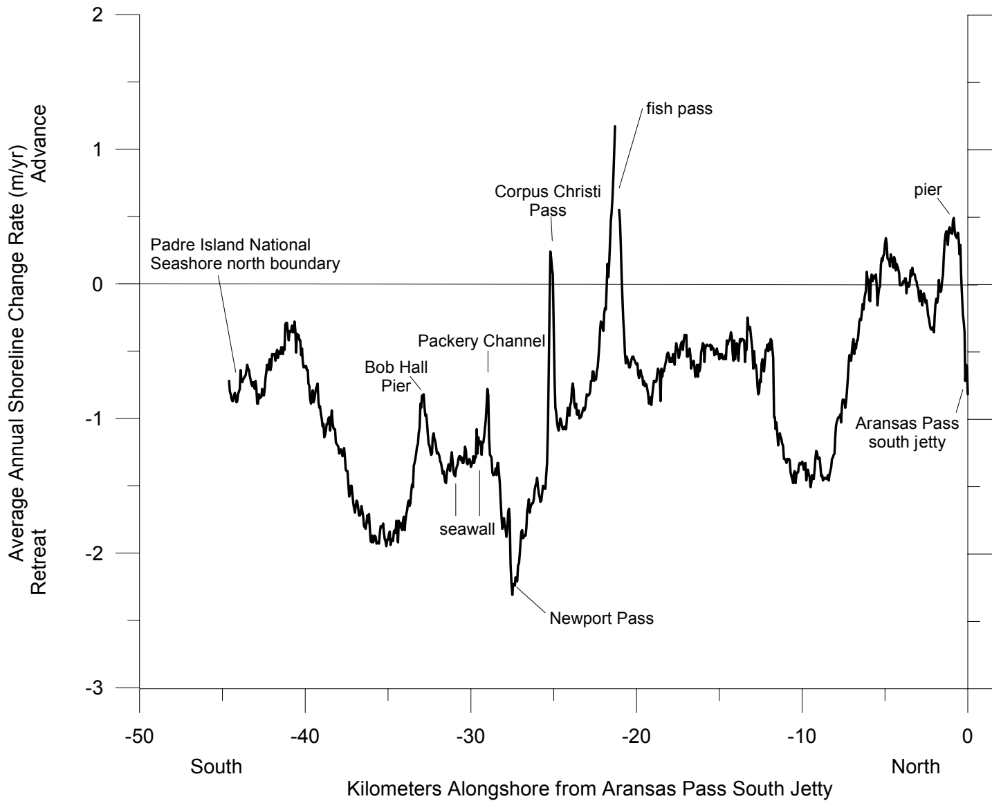
Figure 3. Long-term average annual rate of shoreline change. Six shorelines from 1937, 1956/58/59, 1965/69, 1974, 1990/95, and 2000 were used to determine rate of change based on a linear regression model.
